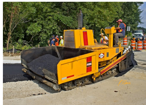
Hot mix asphalt (HMA) paver will place the new road surface
